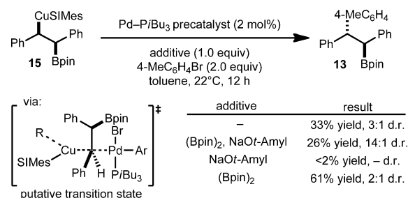
Scheme 5. Study of reaction mechanism for anti -selective conditions.
